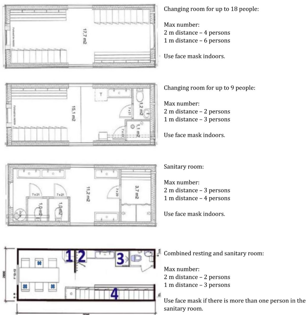
Figure 1 — Examples of the limitations which apply when changing rooms are used at the same time
